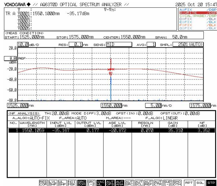
Optical Spectrum of Amplified 1550.12nm signal ( -35dBm input power @95mA current)
